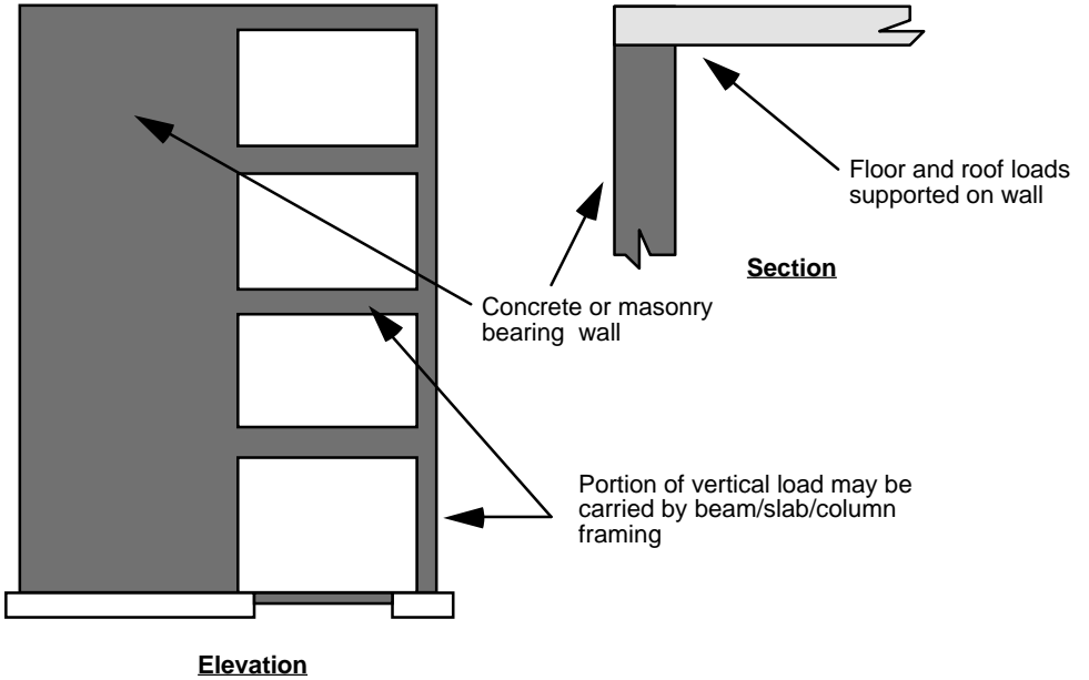
a) Bearing Wall
