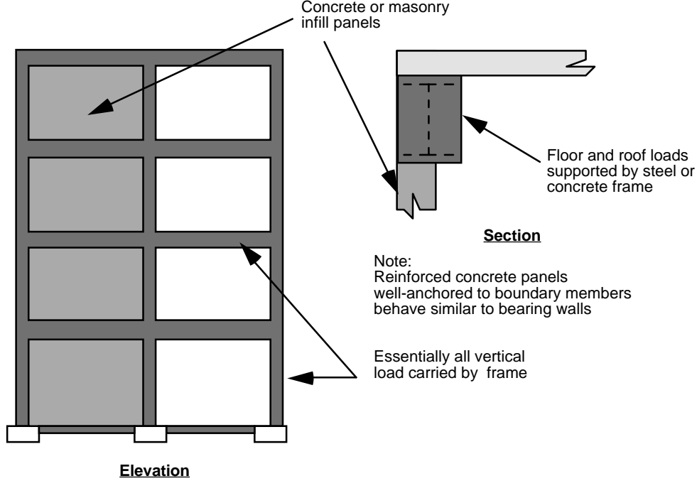
b) Infilled Frame
