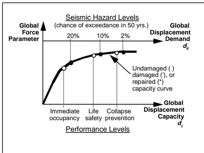
Figure 3-5 Global displacement demands and capacities
