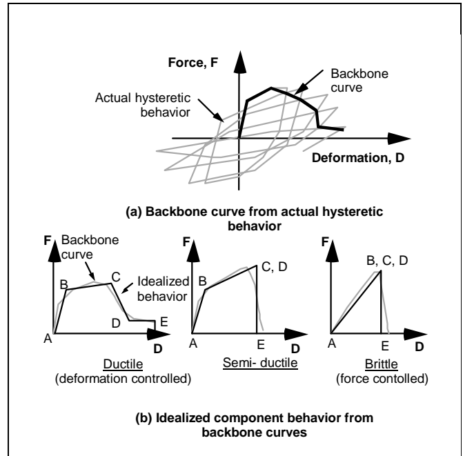
Figure 3-4 Structural component force-deformation characteristics
